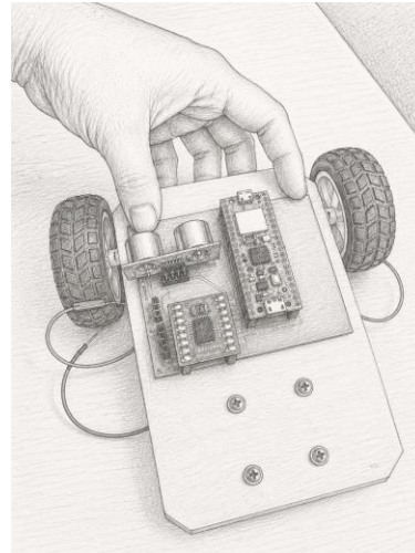
PCB mounted on the chassis
